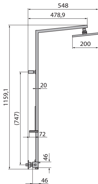
Shower head dimensions / Ducha fija 200 x 200 mm
